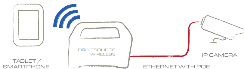
POINTSOURCE Wireless powers the IP camera with POE and provides wireless network access to the camera.
